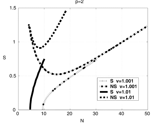
Fig. 4. Dispersion analysis: Plots of the normalized wave number S versus the number of cells per wavelength N , for two levels of accuracy, in the staggered and nonstaggered cases.
