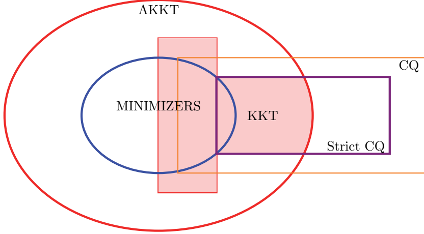
FIG. 1. Optimality relations. Small ellipse: local minimizers . Big ellipse: feasible points that satisfy the AKKT condition . Small rectangle: feasible points that satisfy an SCQ . Big rectangle: feasible points that satisfy a (not necessarily strict) CQs . Shaded area: KKT points .
