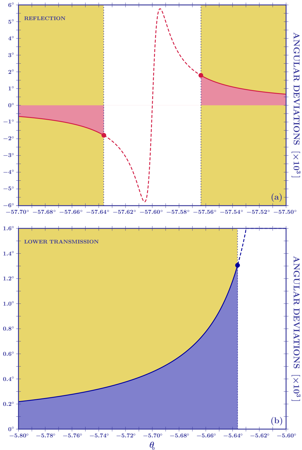
Figure 3: For a BK7 prism and incident laser beam with \lambda = 0.633 \mu\text{m} and waist w_0 = 1 \text{ mm} , the Brewster region for external reflection and the critical region for the lower transmission are plotted in (a) and (b), respectively. In (a) the amplification is proportional k w_0 producing the so-called giant GH angular shift while in (b) it is proportional to 1/k w_0 . The white background indicates the region where the concept of angular deviation is obscured due to the presence of an additional peak in the angular distribution of the reflected beam (a) or to the complex nature of the reflection coefficient (b).
