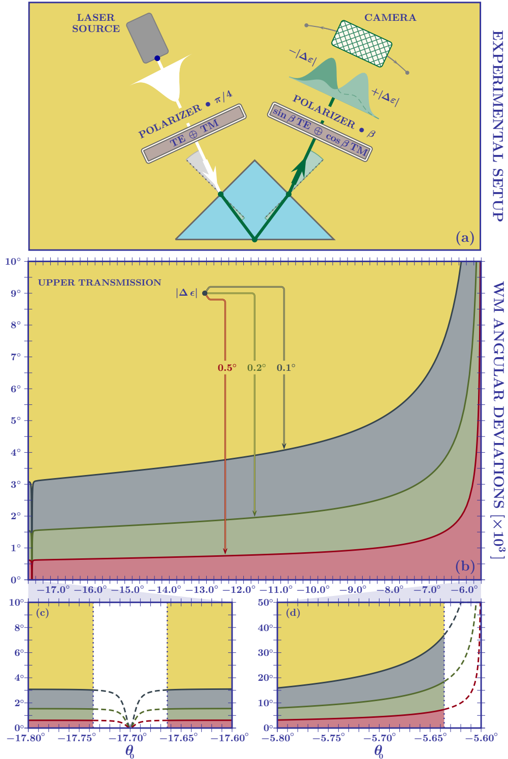
Figure 6: In (a), the weak measurement (WM) experimental set-up is displayed. For angular settings of the second polarizer, |\Delta\epsilon| = 0.1^\circ, 0.2^\circ, 0.5^\circ , we respectively find amplifications proportional to 1/|\Delta\epsilon| , see (b). Approaching the critical angle, we find a global additional amplification. This is clearly shown in the insets (c) and (d) where we zoom to the Brewster (c) and the critical (d) regions. The breaking off of the giant GH angular shift near the Brewster region is clearly visible in (c) and the global amplification of a factor 10 optimizing the WM analysis bear the critical angle in (d).
