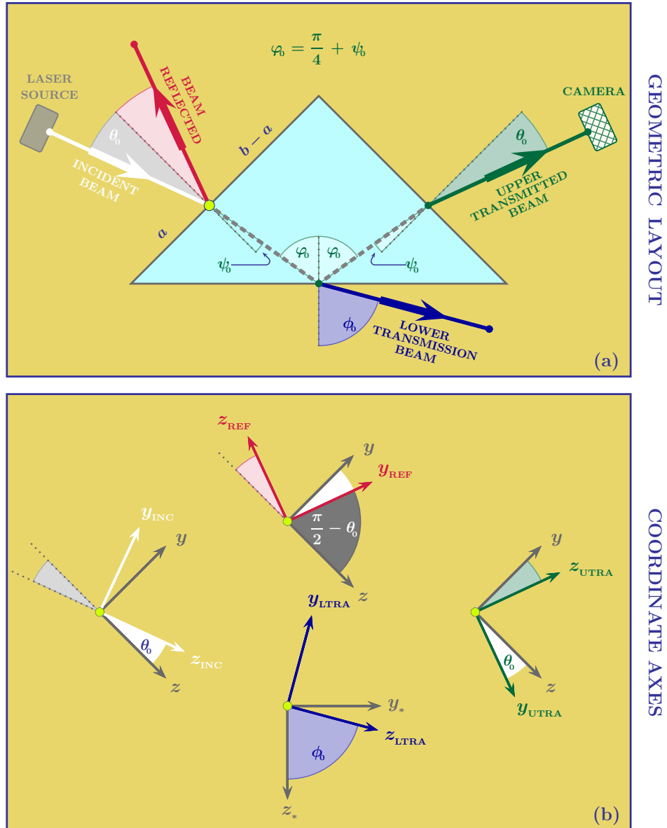
Figure 1: Planar view of the dielectric block used for the analysis carried out in this paper. The incidence angle at the lower (dielectric/air) interface, \varphi_0 , is always positive and given by \pi_0/4 + \psi_0 ( \sin \theta_0 = n \sin \psi_0 ). In (b), the axes describing the propagation of the incident (INC), reflected (REF) and transmitted (TRA) beams are displayed.
