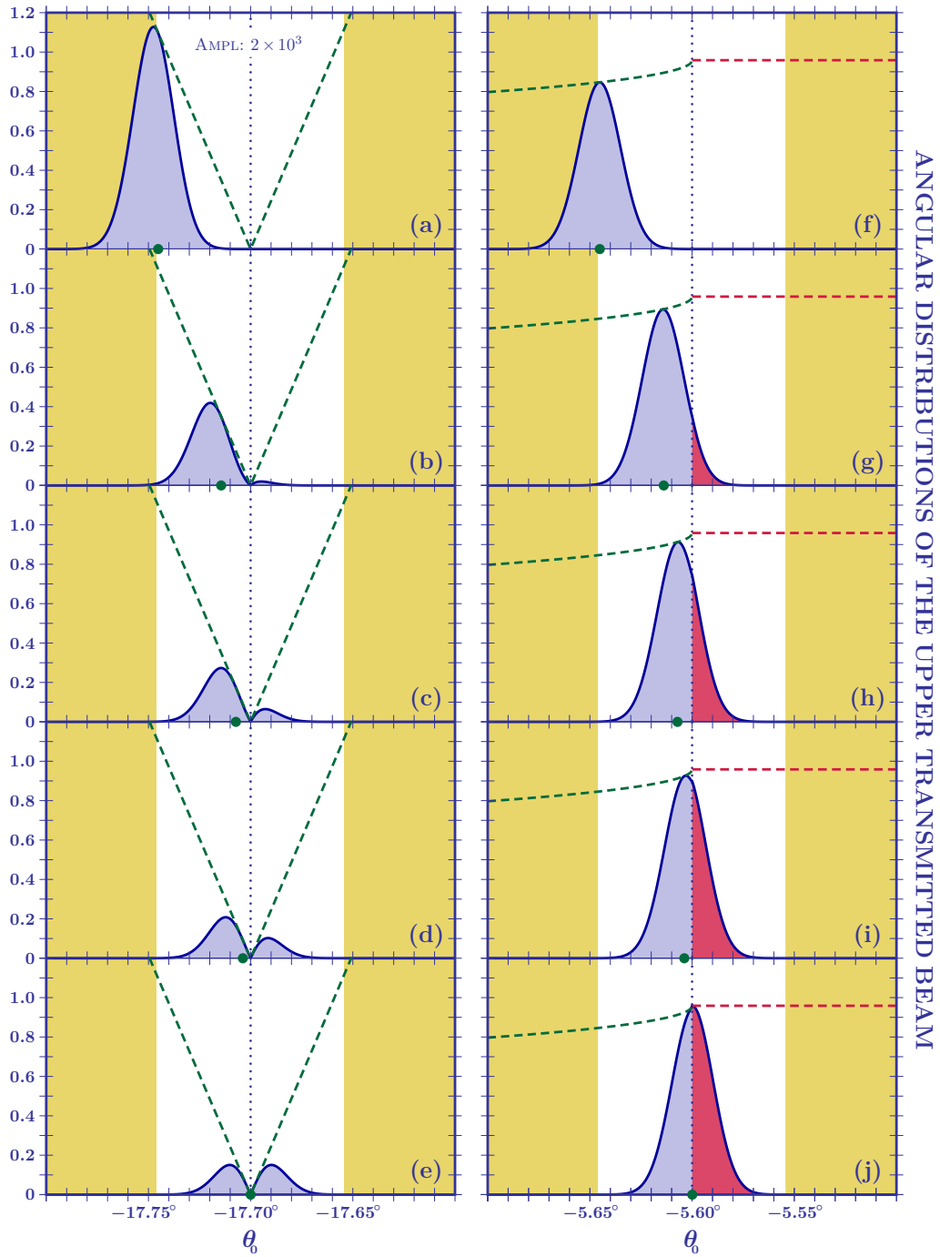
Figure 5: Angular distribution absolute values of the transmitted beam in the Brewster (a-e) and critical (f-j) regions. The dashed lines represent the absolute values of the Fresnel coefficients. The concept of angular deviation works for incidence at \theta_{B(\text{int})} - \lambda/w_0 (a) and \theta_{\text{cri}} - \lambda/w_0 (f). For incidence approaching the Brewster and critical angles, the presence of an additional peak, see insets (b-e), and of a complex angular distribution, red zone in (g-j), obscure the concept of angular deviations.
