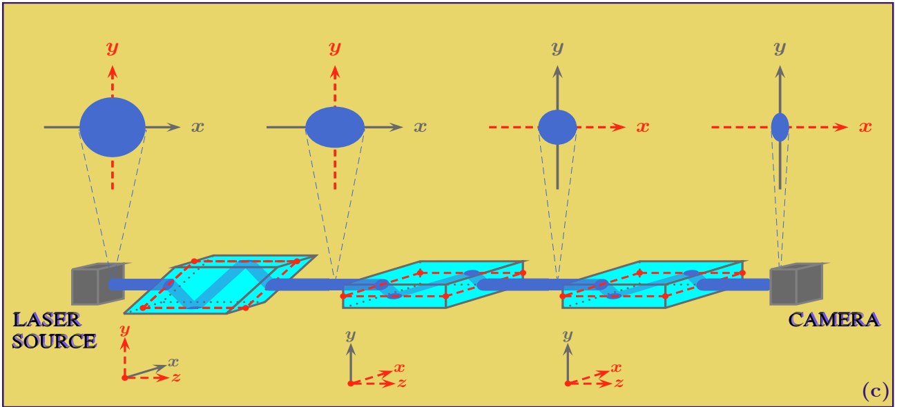
Figure 1: Experimental setup. The incoming beam propagate along the z -axial forming an angle of \pi/4 with the left interface of the dielectric blocks. In (a), the plane of propagation is the plane y - z and represents the configuration (M, N) = (0, 1) . In (b), the block is clockwise rotated by an angle \pi/2 along the axial axis, configuration (M, N) = (1, 0) . In (c), we have the configuration (M, N) = (2, 1) . The transversal symmetry is recovered when the beam passes through the same number of blocks M and N .
