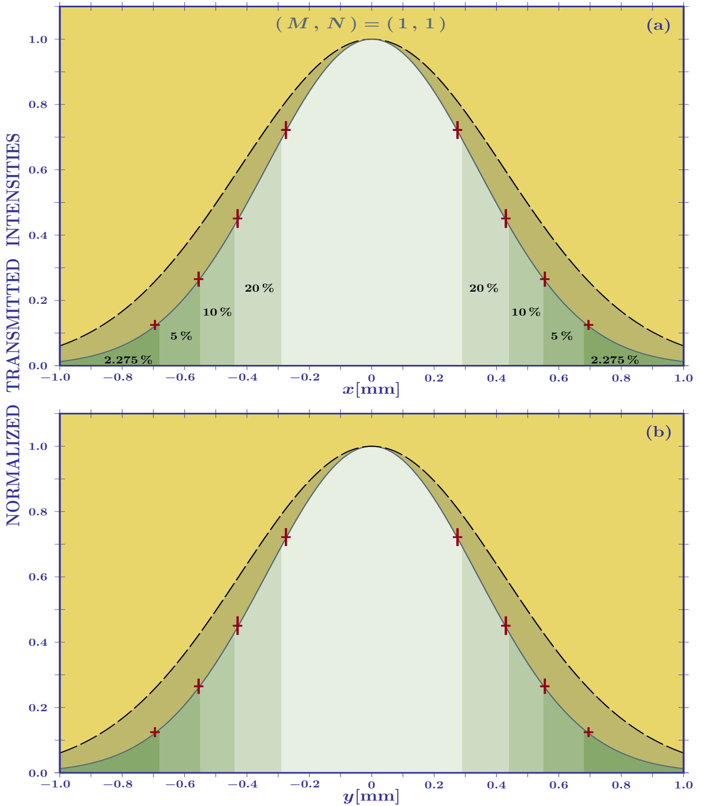
Figure 3: Transversal profiles of the normalized transmitted intensity. The dashed black lines represent the profiles for free propagation. The blue solid lines are the profiles for beams passing through the dielectric configuration (M, N) = (1, 1) . The symmetry between the transversal components x and y is recovered. It is also possible to see the axial spreading delay with respect to the free propagation. The experimental data show an excellent agreement with the theoretical curves.
