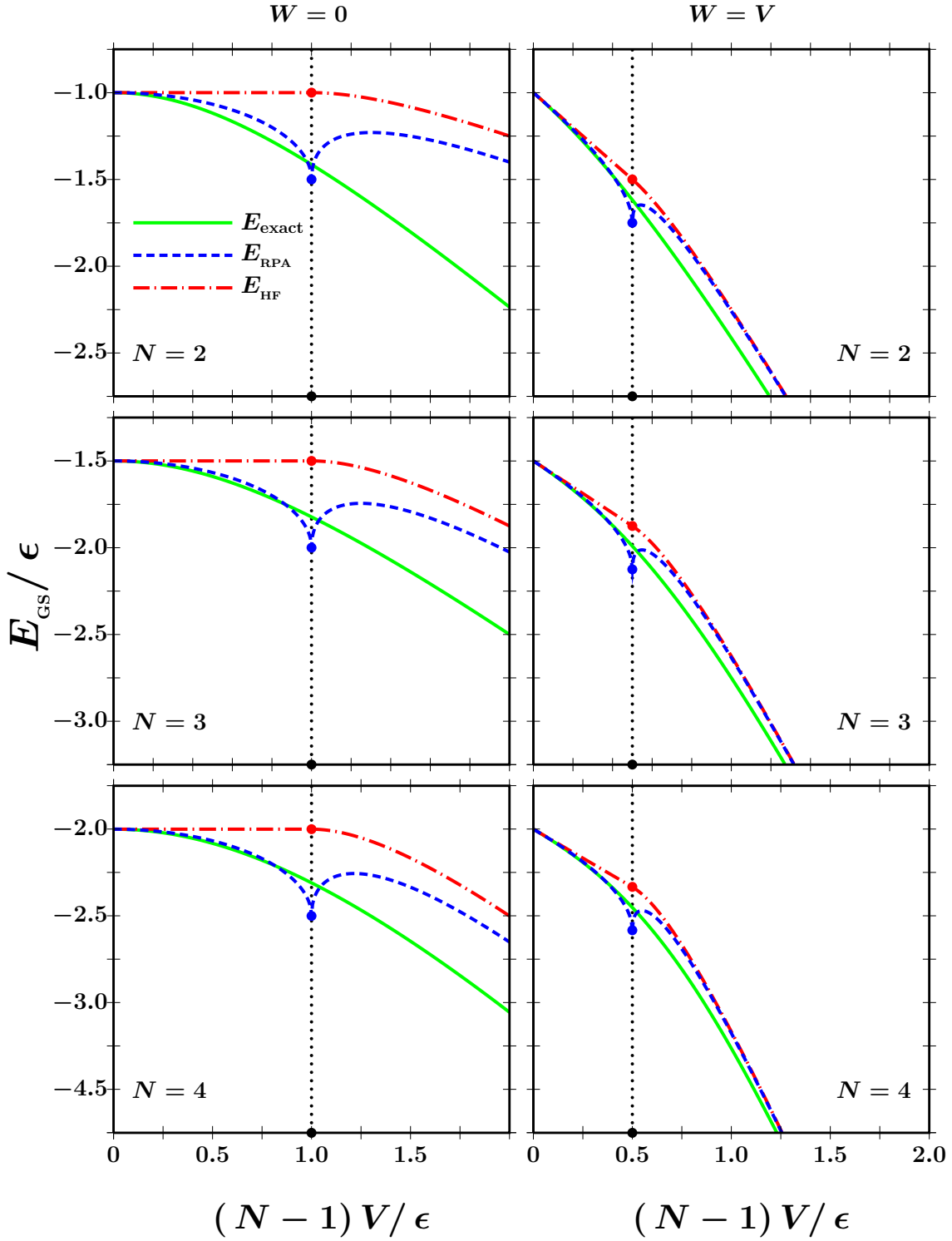
FIG. 1. Ground state energies as a function of the interaction strength V for systems composed by N = 2, 3 and 4 particles. The full (green) lines indicate the solutions obtained without approximations. The dash-dotted (red) lines the results obtained with the HF model, and the dashed (blue) lines those obtained with the RPA approach. The left panels show the results for W = 0 , and the right panels those obtained by setting W = V . The blue and red thick dots emphasize the values of the HF and RPA energies in the discontinuity line.
