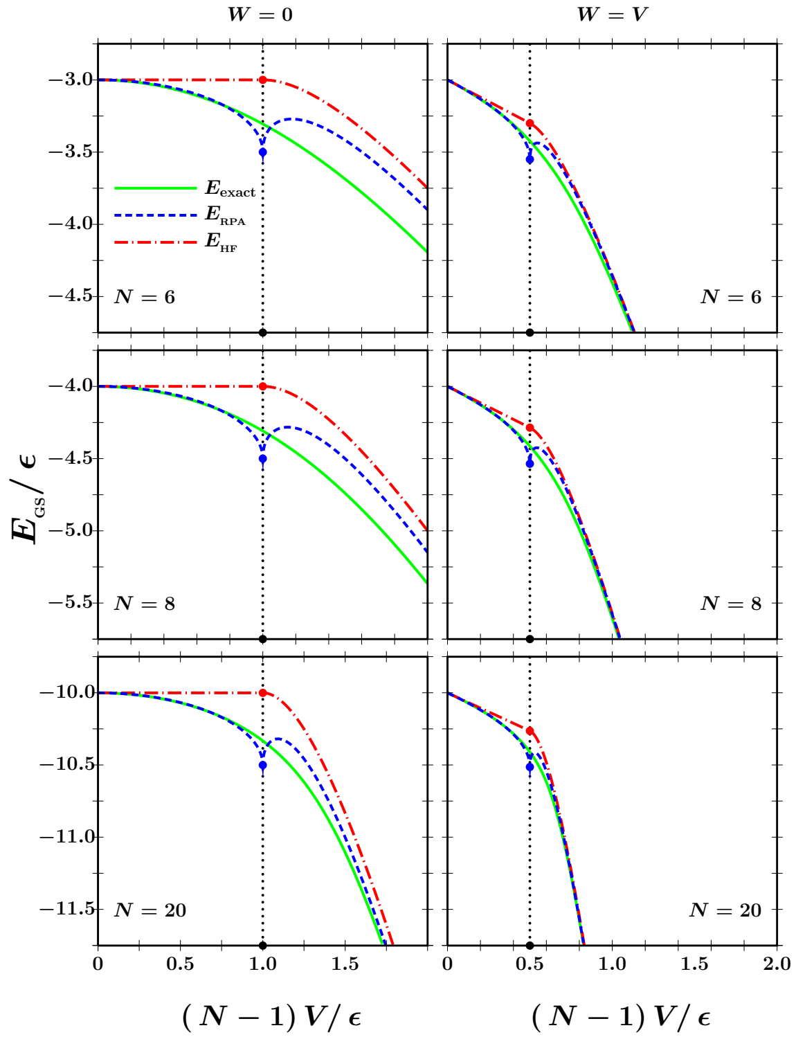
FIG. 2. The same as in Fig. 1 for N = 6, 8 and 20 .
