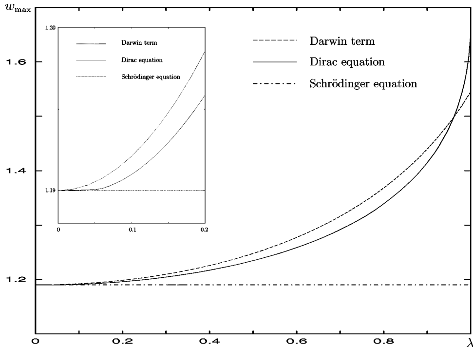
FIG. 2. Comparison of w_{\max} against \lambda for the ground state in the Dirac and Schrödinger equations. The dashed curve is the magnification effect of the Yukawa version of the Darwin term alone.
