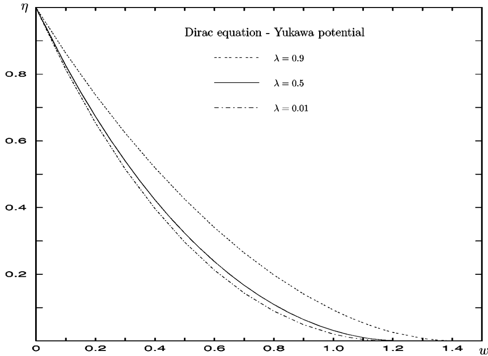
FIG. 1. \eta versus w for the ground state of the Yukawa potential in the Dirac equation. Three values of \lambda are shown. For \lambda \ll 1 (the dot-dashed curve) we reproduce essentially the Schrödinger equation result. The value of w_{\max} when \eta=0 shows an increase with increasing \lambda .
