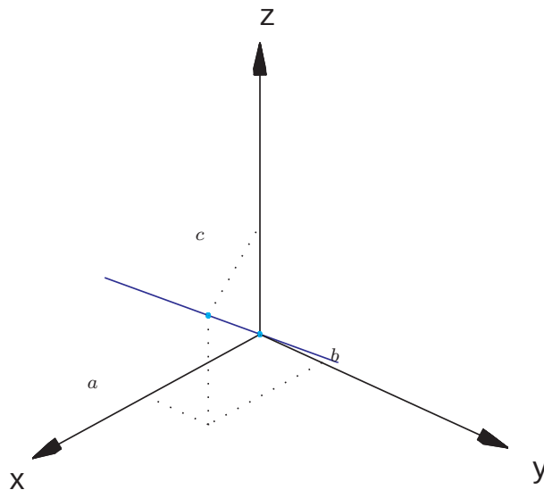
Figura 4.16: Reta (x, y, z) = (at, bt, ct)
