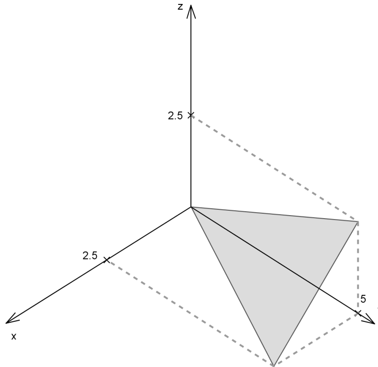
Figura 4.21: \pi_2 : 2x - y + 2z = 0
