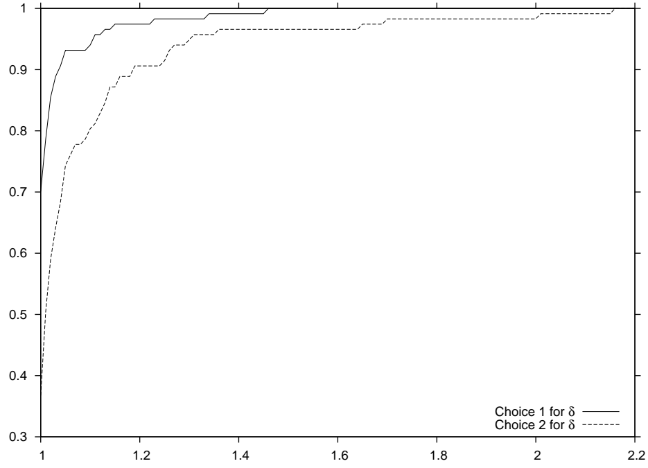
Figure 1: Performance profile comparing choices 1 and 2 of the Partial SPG parameter \delta^k .
